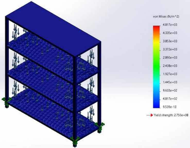
RACK FOR HEAVY MATERIAL SLDPRT-Static 3-Stress-Stress1
